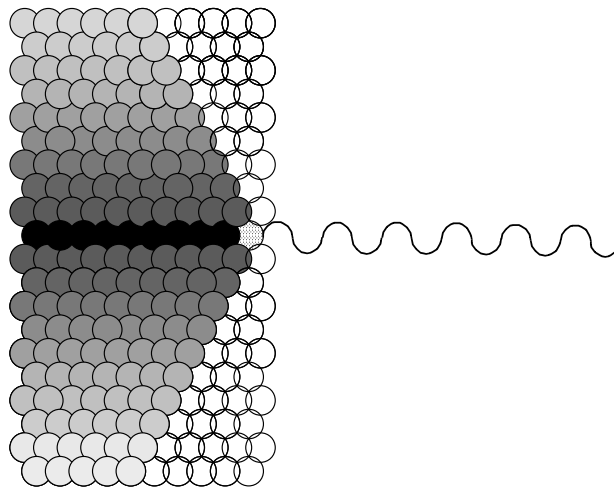
Figure 35 (Left) A linear-radial distortion complex. (Right) An electromagnetic wavicle. Within the context of the relational-matrix model, electromagnetic radiation is analogous to the linear component of the linear-radial distortion complex. As explained earlier, the pattern of distortion content represented by the linear component of the linear-radial distortion complex is that of a maximal distortion.
