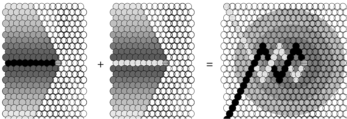
Figure 55 The mass of the matter is most obviously and directly related to the number of primary distortion processes that are stably and repetitively interacting to compose the compound process as a whole. The two drawings to the left show two linearly propagating primary distortion processes (black and stippled circles). As those two primary distortion processes stably and repetitively interact to form a compound process or matter, the gravitational distortions (gray areas) associated with each component process additively overlap, creating a relatively greater gravitational distortion, both internal and external to the compound process. The more primary distortion processes interact to compose the matter, the greater is the additive overlap of the gravitational distortions, internally increasing the inertial field and externally increasing the gravitational field, resulting in the measurement of a larger mass for the material object, since mass is a measure of the inertial property of matter. However, since mass varies with material velocity, mass must represent more than just the simple summation of the gravitational distortions associated with the component processes.
