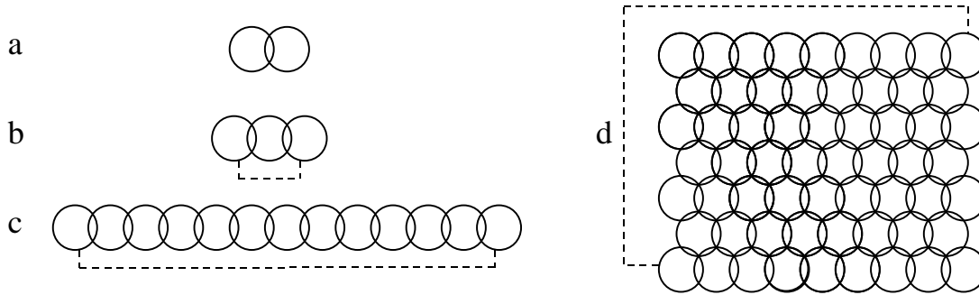
Figure 58 How reality cells that are spatially separate have a connection that transcends spatial distance. Implicit in the existence of each reality cell is the existence of the reality cells it exists in relation to. This shared existence between adjacent reality cells is depicted by the overlap between adjacent reality cells. In figure a, it's evident that each reality cell shares part of its existence with the adjacent reality cell. However, because of this shared existence between adjacent reality cells, there's also a shared existence between reality cells that aren't directly adjacent to one another, as depicted in figure b. That is, the reality cell on the far left in figure b contains part of the existence of the reality cell on the far right, because the reality cell between them, which seems to separate them, contains some of the existence of each. Essentially, what exists here also exists there, although there seems to be something else in between. This logic can then be extended to reality cells that have many intervening reality cells between them, as depicted in figure c. In figure c, the two reality cells at each extreme share part of their existence, because all of the reality cells between them contain some of the existence of all the others. Again, what exists here also exists there, although there seems to be something else in between. This shared existence between reality cells implies an underlying unity that defies the apparent spatial separation between them. In figure d, this logic is applied to the two-dimensional relational-matrix diagram to show that all reality cells share existence and thus are connected in a way that defies spatial separation.
