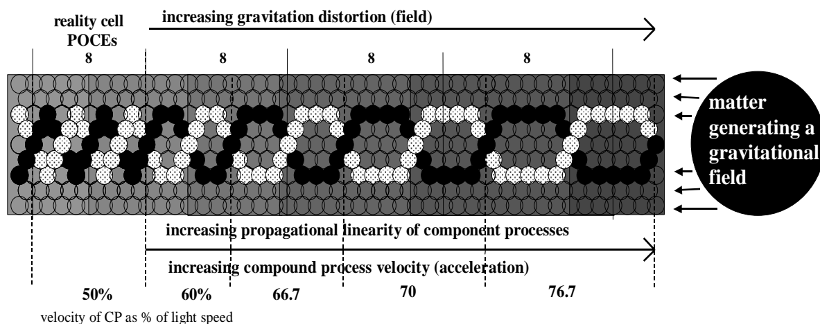
Figure 49 A compound process (CP) that is accelerating, owing to a gravitational field that’s being generated by, and exists in association with, the matter on the right. As the CP encounters the gravitational field, the direction of propagation of its component processes (black and stippled circles) is altered in the direction of increasing gravitational distortion (increasingly dark shades of gray from left to right), increasing the degree of linearity of propagation of the component processes, and thus both increasing the velocity of the CP as a whole and attracting it in the direction of the matter that’s generating the gravitational field. This increase in velocity (i.e., acceleration) moves the CP into an even stronger gravitational distortion, further increasing the degree of linearity of propagation of the component processes, again both increasing the velocity of the CP as a whole and attracting it in the direction of the matter that’s generating the gravitational field, and so on. The continuous repetition of this cycle is what we observe as gravitational acceleration.
