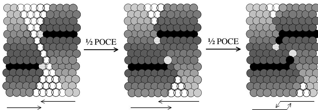
Figure 41 The gravitational basis of primary-distortion-process interaction, depicted here as the mutual alteration of the direction of propagation of each primary distortion process’ linear electromagnetic component by the other’s radial gravitational component. Depicted here are two primary distortion processes, each composed of a linear electromagnetic distortion (black areas) and a coexistent radial gravitational distortion (gray areas). The electromagnetic distortion propagates linearly through the relational structure of space-time, leaving a radially propagating gravitational “wake” in its path. When two primary distortion processes come into proximity, each’s direction of propagation can be affected by the other’s gravitational “wake,” such that the direction of propagation of each’s linear electromagnetic component is altered toward the direction of propagation of the other’s.
