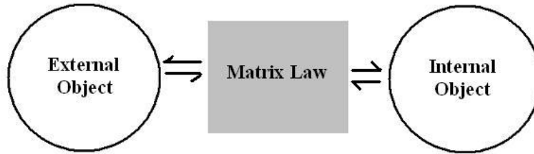
Figure 2.3 Self-interaction between external and internal objects of a quantum entity in a dual universe comprised of an external spacetime and an internal energy-momentum space, vice versa .
