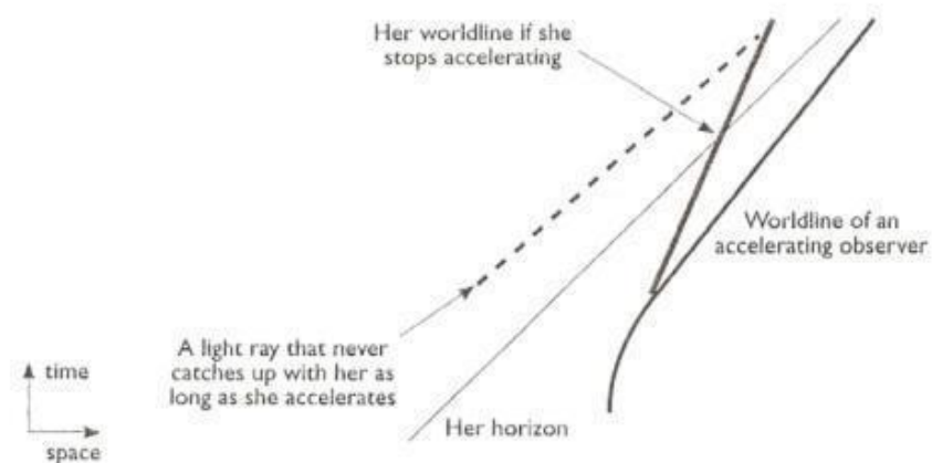
Accelerating Observer's Horizon (image from Smolin)
