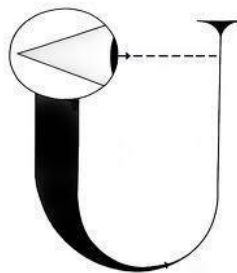
Wheeler's Universal Observer (image from cosmoquest.org)
