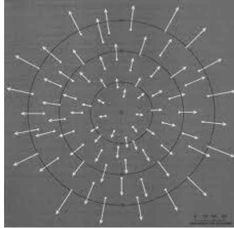
Accelerated Expansion of Space (image from Susskind)
