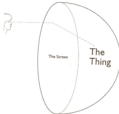
The Observer, the Screen and the Thing (image from Smolin)
