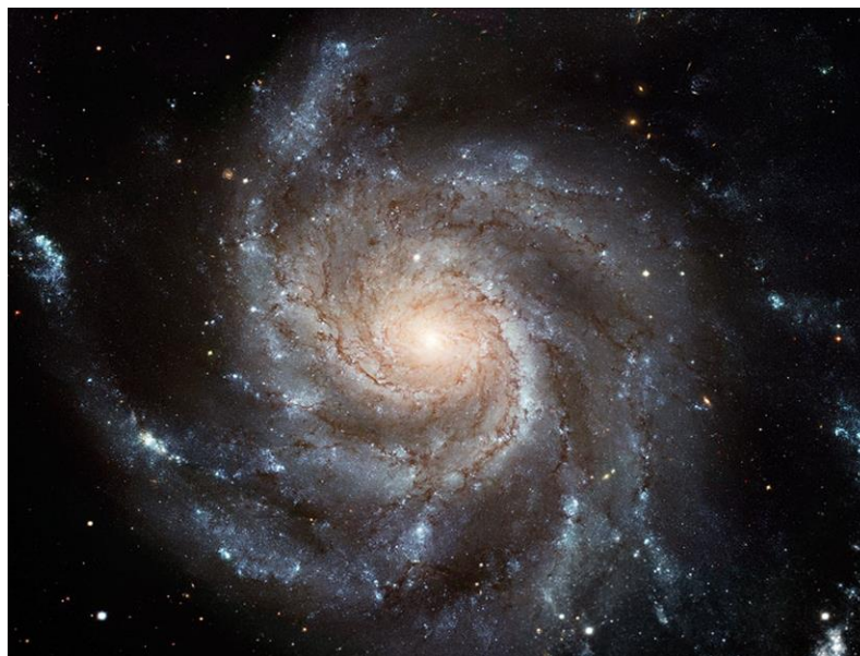
Fig. 5. Hubble Space Telescope Image of Spiral Galaxy M101 (courtesy NASA).
